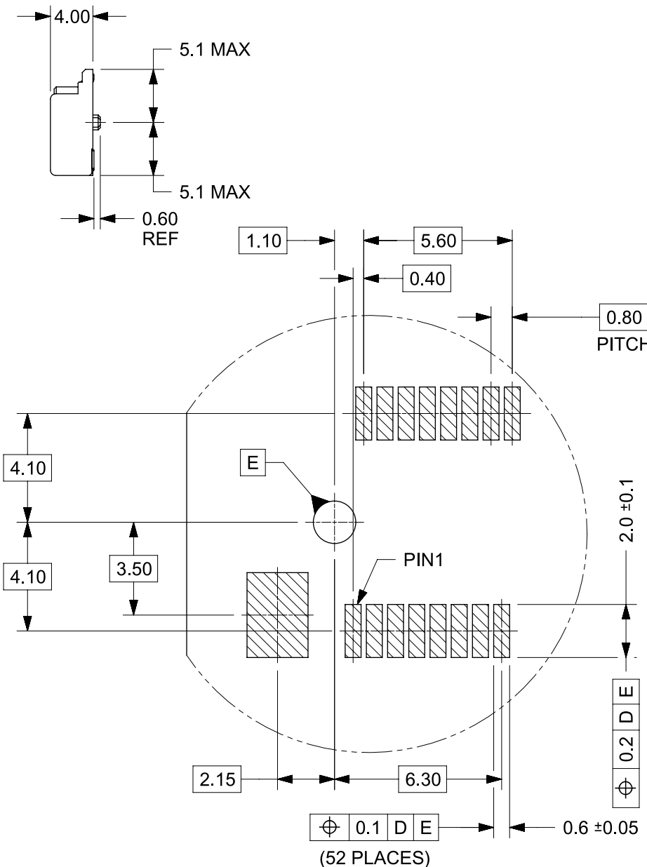
DETAIL B SCALE 5:1
