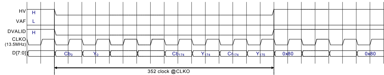
Timing Chart (Camera I/F) QCIF (NTSC) Register Set : VLF = 1'b0, OFORM[2:0] = 3'b011, OIF[1:0] = 2'b00
