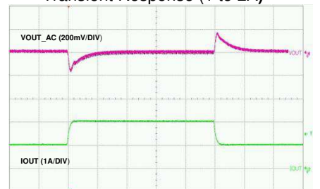
Transient Response (1 to 2A)
