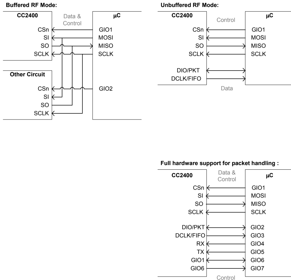
Figure 8. Microcontroller interface
