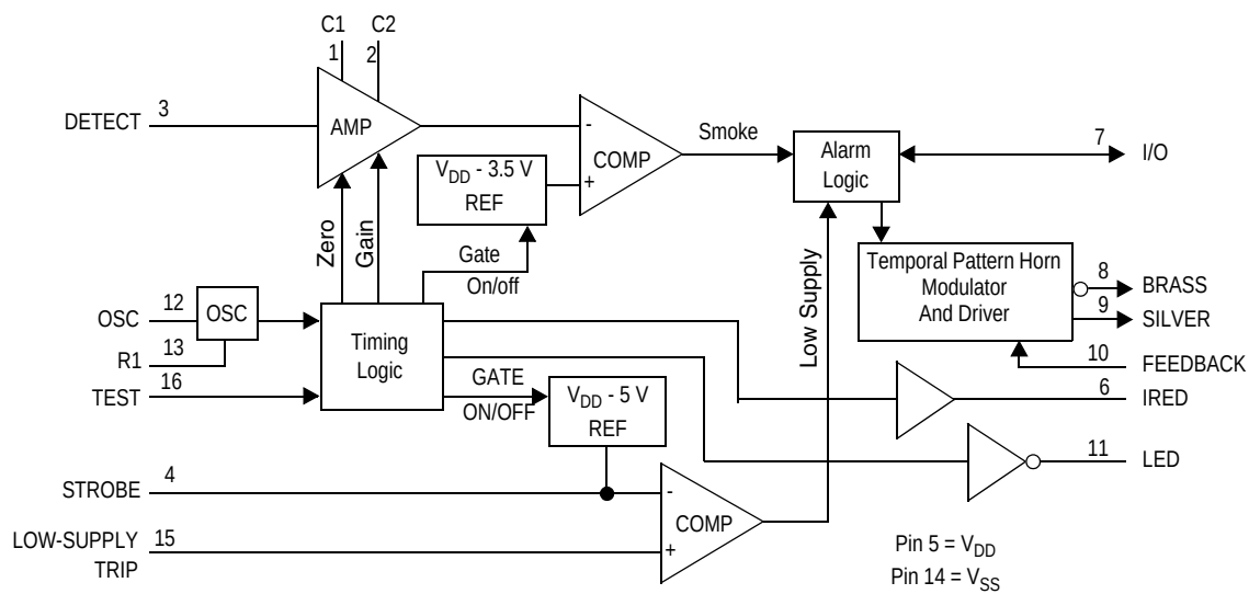
Figure 2. Block Diagram
