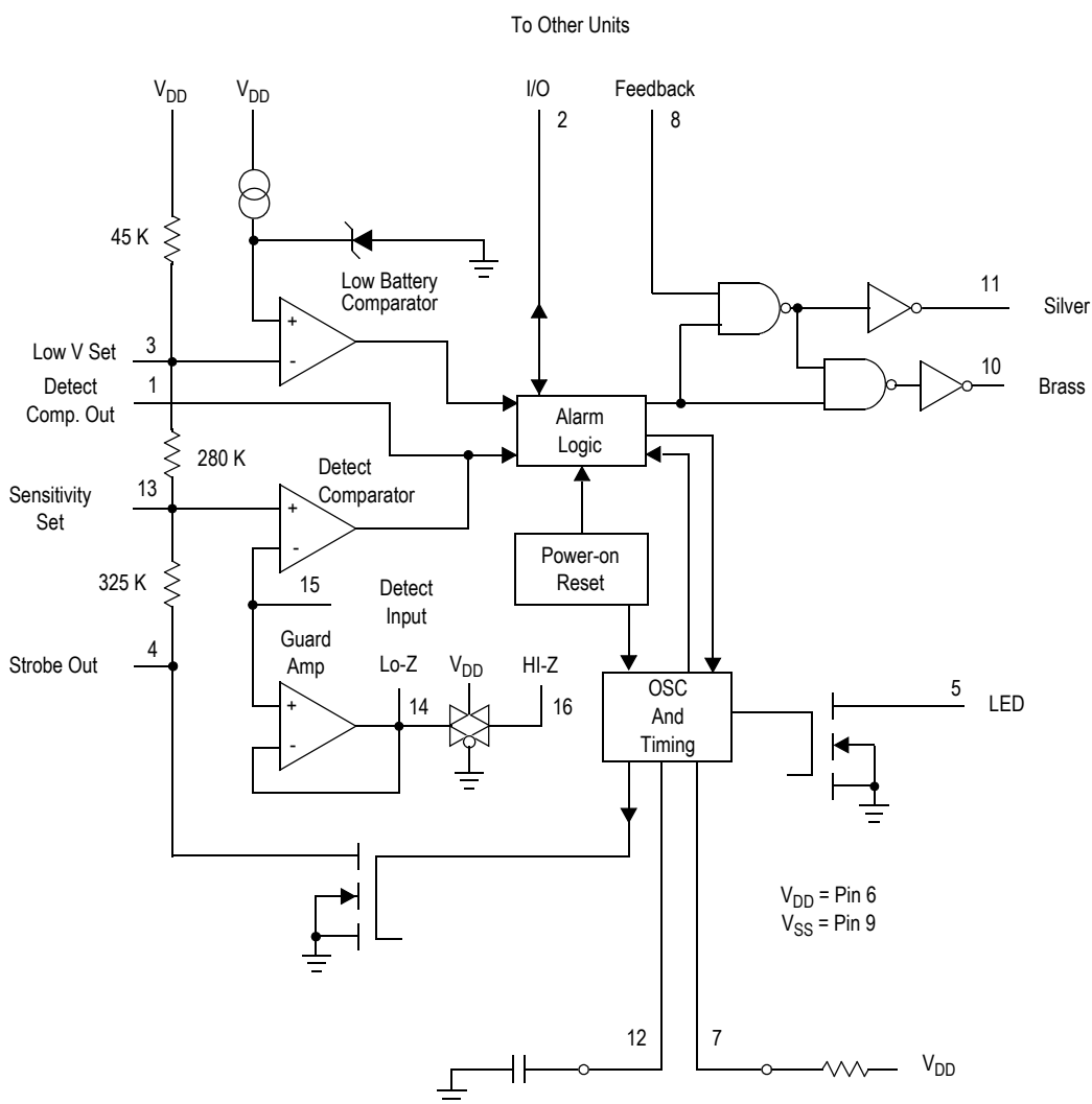
Figure 2. Block Diagram
