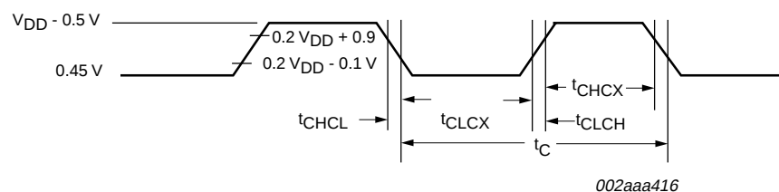
Fig 27. External clock timing.
