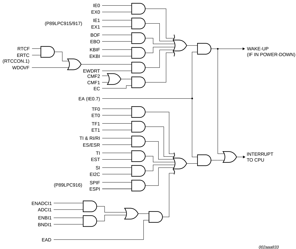
Fig 12. Interrupt sources, interrupt enables, and power-down wake-up sources.
