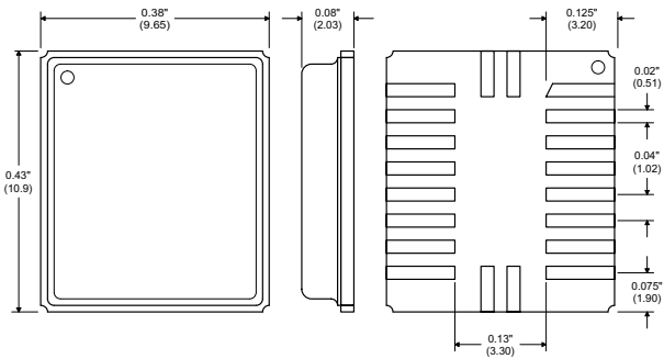
SM-20L Package Drawing
