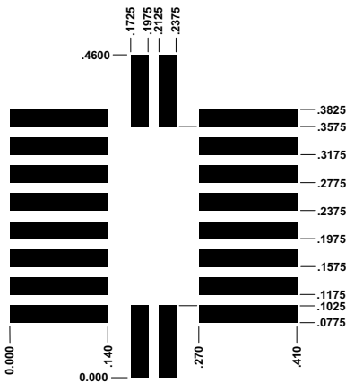
Dimensions in inches SM-20L PCB Pad Layout
