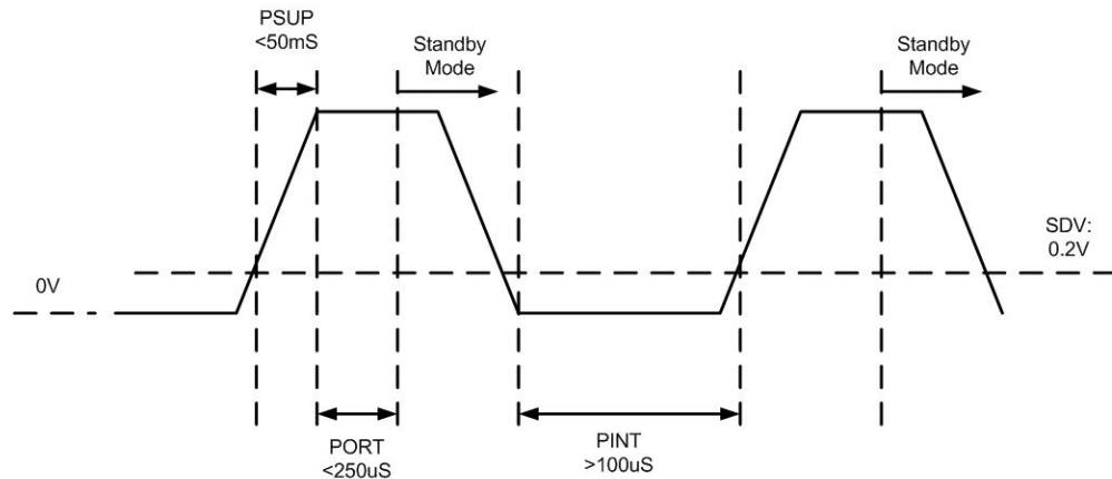
Figure 9. Power On/Off Timing
