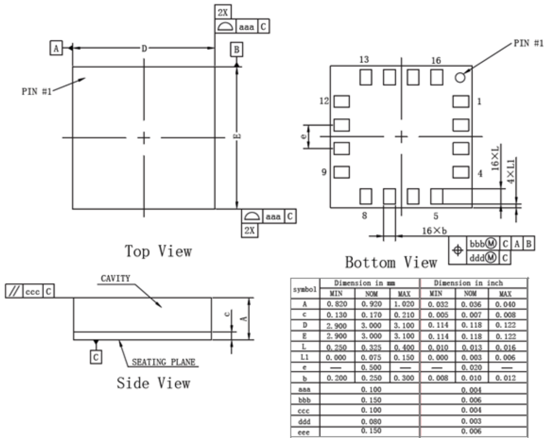
Figure 4. Package Size
