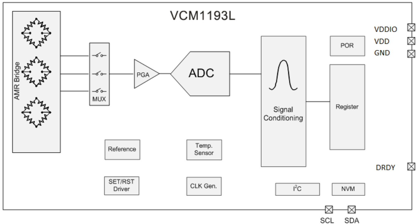
Figure 1. Block Diagram
