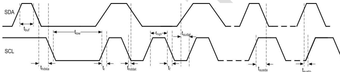
Figure 11. I 2 C Timing Diagram
