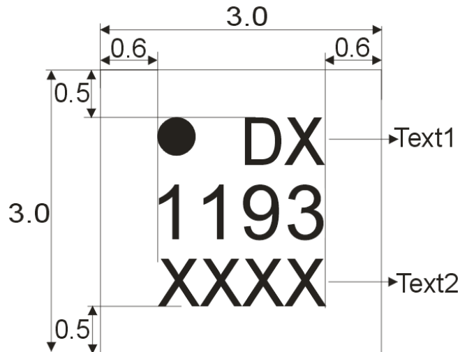
Figure 5. Chip Marking
